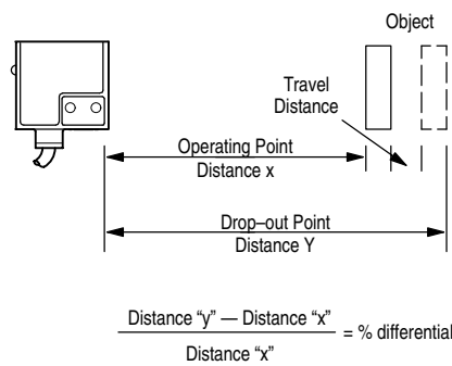
Figure 19 Hysteresis
