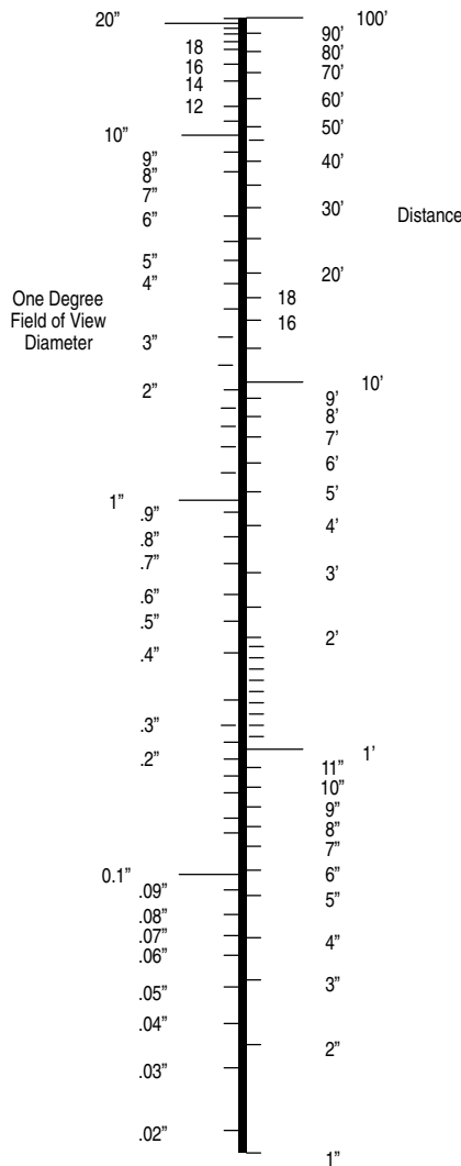
Figure 17 Field of View Diameter vs. Distance
